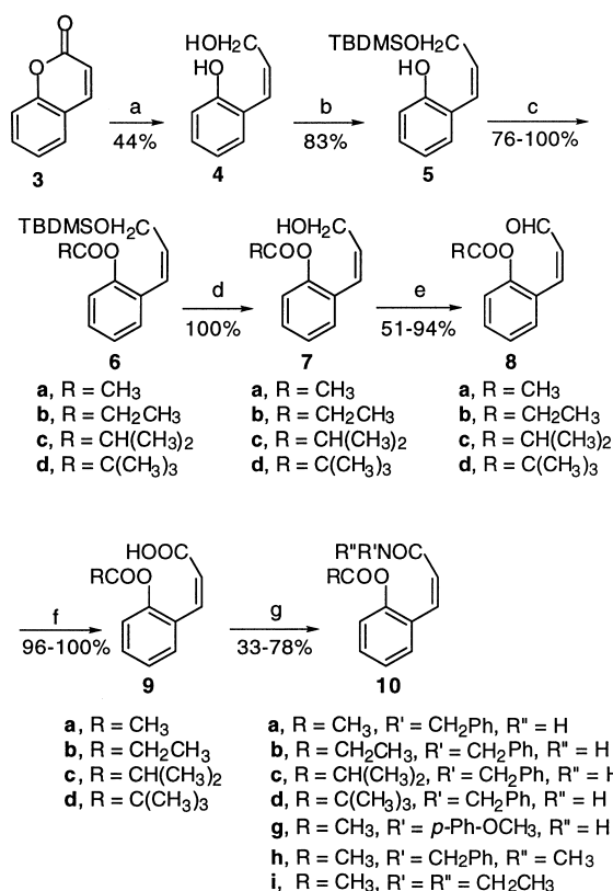
Scheme 2. Synthesis of the coumarin-based model prodrugs 10a-i . Reagents and conditions: (a) LAH, 0 °C, 15 min; (b) TBDMSCl, DMAP; (c) (RCO) 2 O, DMAP-TEA; (d) H 2 O:THF:HOAc (1:1:3); (e) PCC or MnO 2 ; (f) H 2 O 2 , NaClO 2 , 10 °C; (g) DCC/HOBt, DMAP, HNR'R''.
